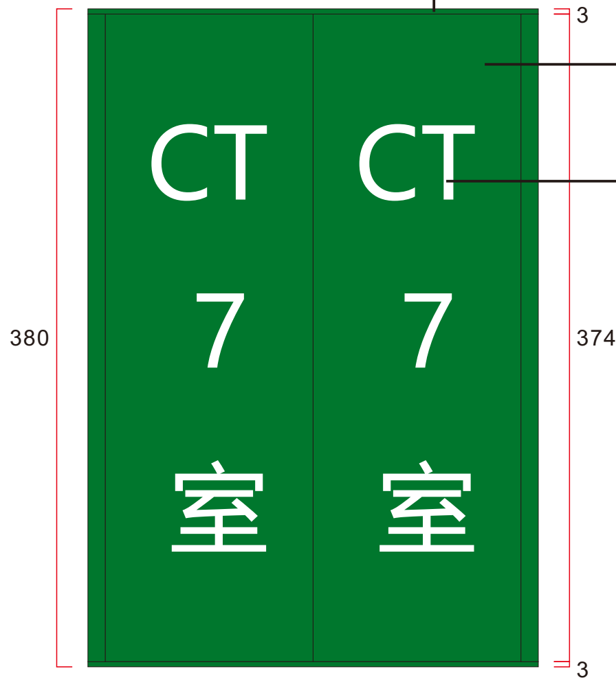
面板展开
